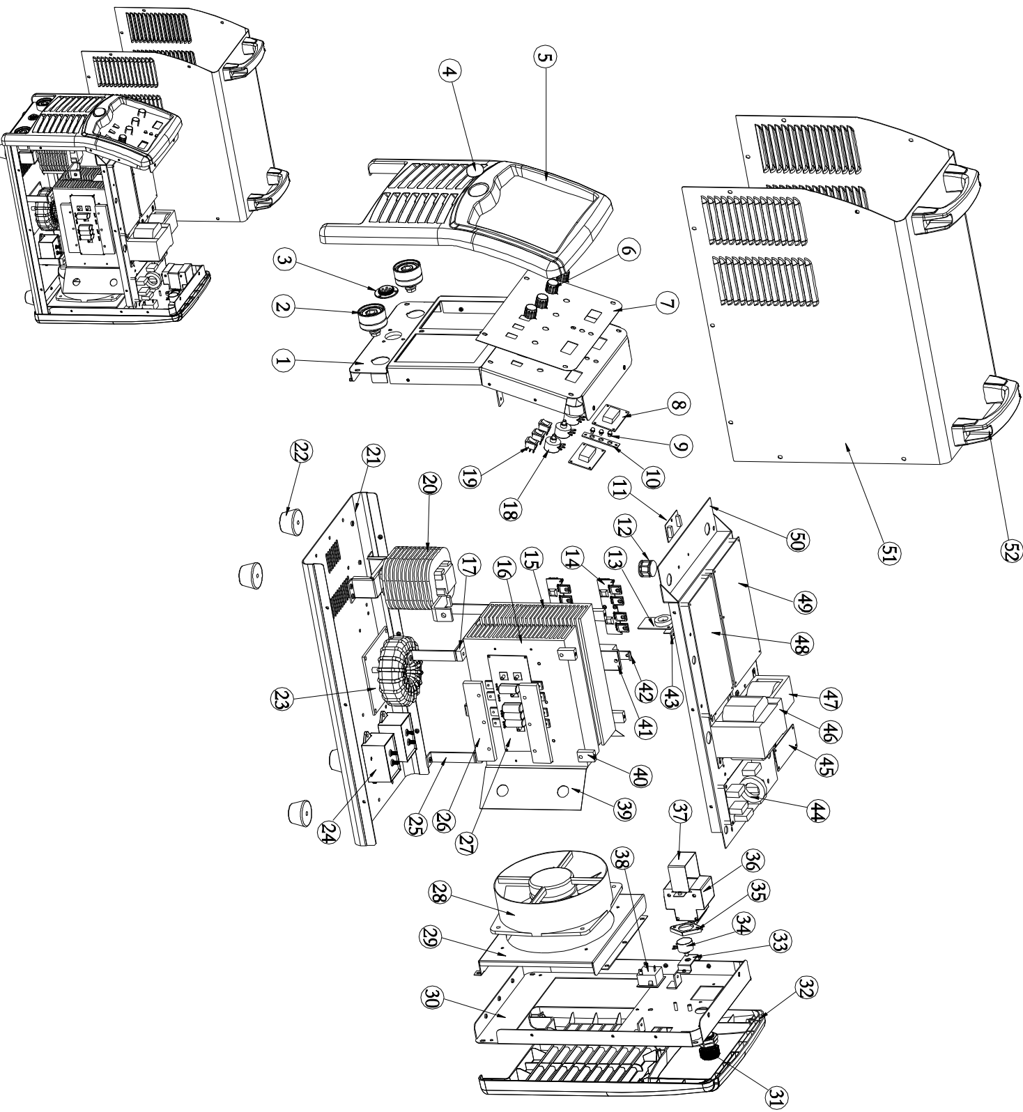
MIG500 explosive view N221-EV
